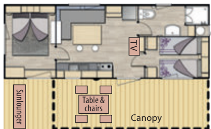
The Murano - 8m long x 3m wide
